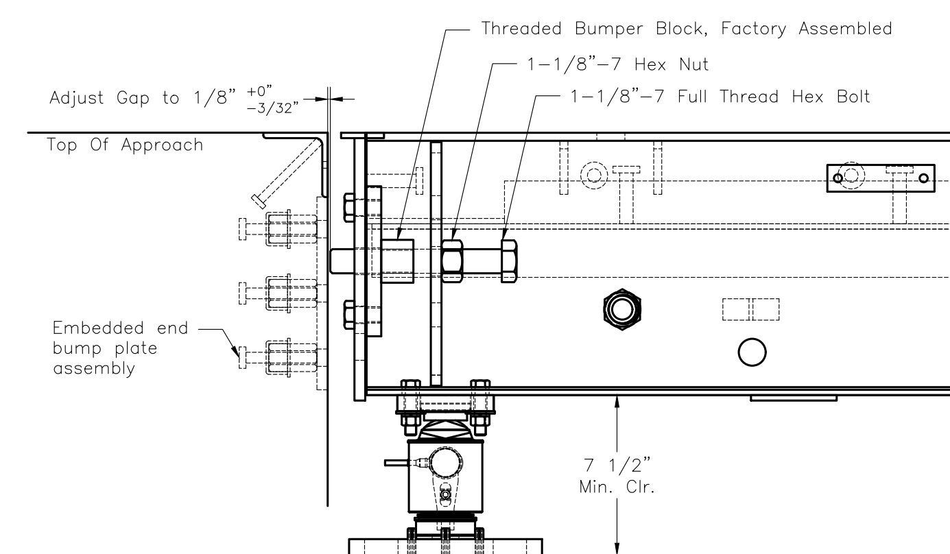
END CHECKING DETAIL Note: Side checking hardware not shown in this view for the sake of clarity
